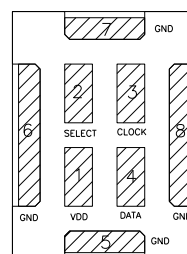
Pin configuration (Bottom view)
