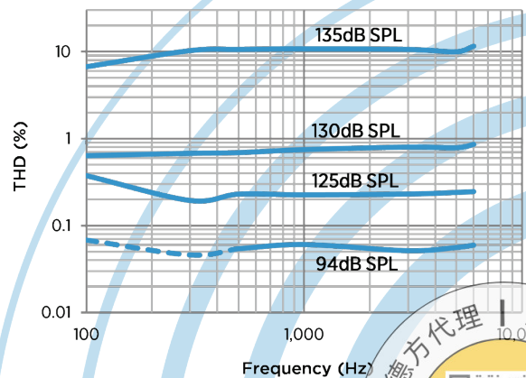
Figure 5: Typical THD vs Frequency
