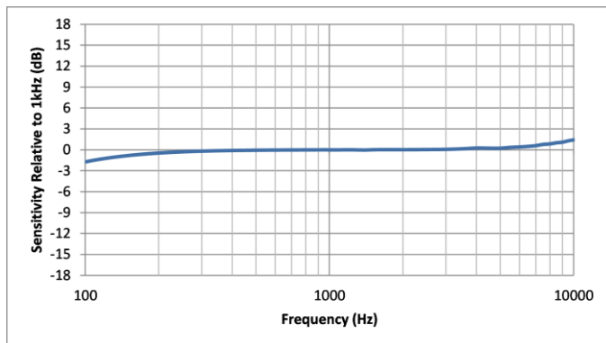
Figure 3: Typical Free Field Magnitude Response and Mask
