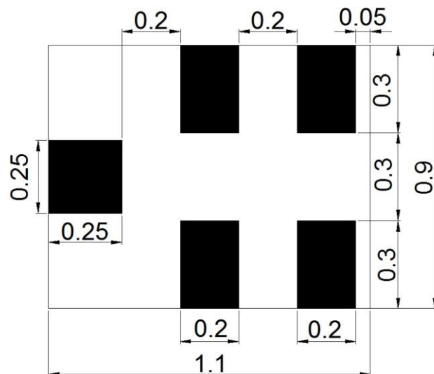
[PCB, X-ray Top view]
