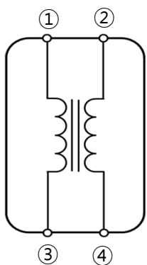
[ EQUIVALENT CIRCUIT ]
