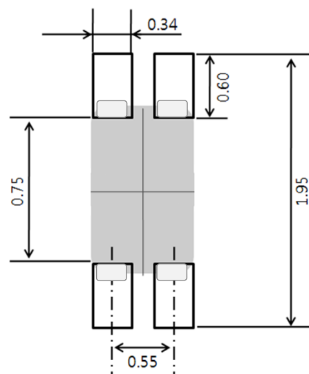
[ Stencil Mask ]
